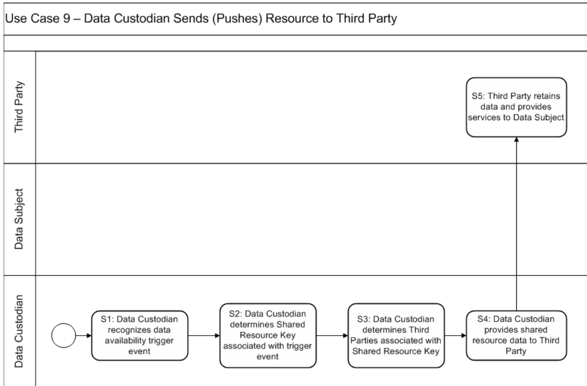
Diagram: Use Case 9 – Data Custodian Sends (Pushes) Resources to Third Party
