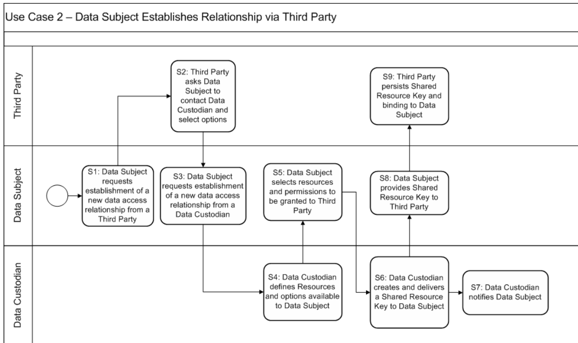
Diagram: Use Case 2 – Data Subject Establishes Relationship via Third Party
