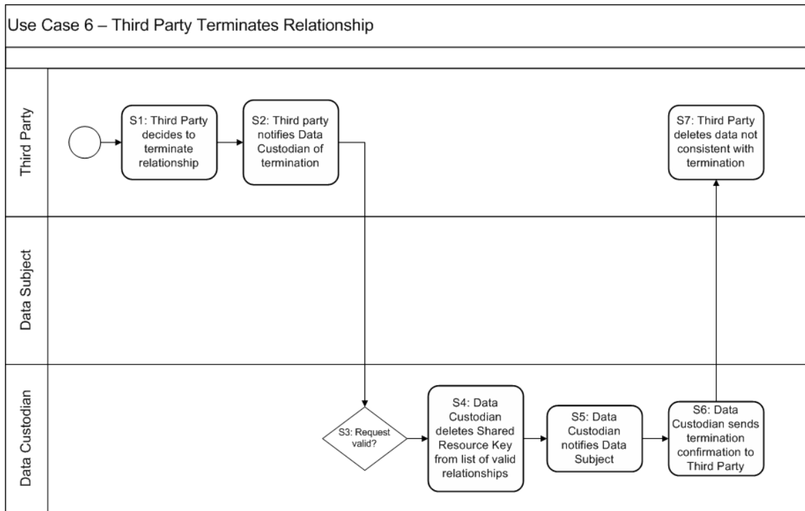
Diagram: Use Case 6 – Third Party Terminates Relationship
