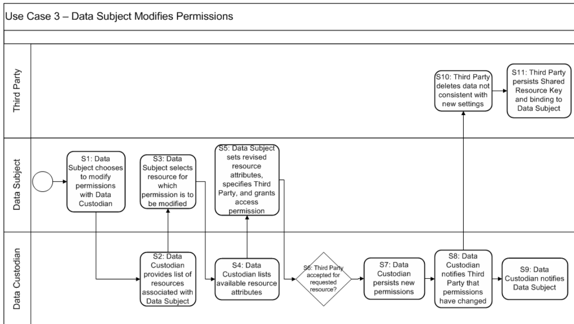
Diagram: Use Case 3 – Data Subject Modifies Permissions
