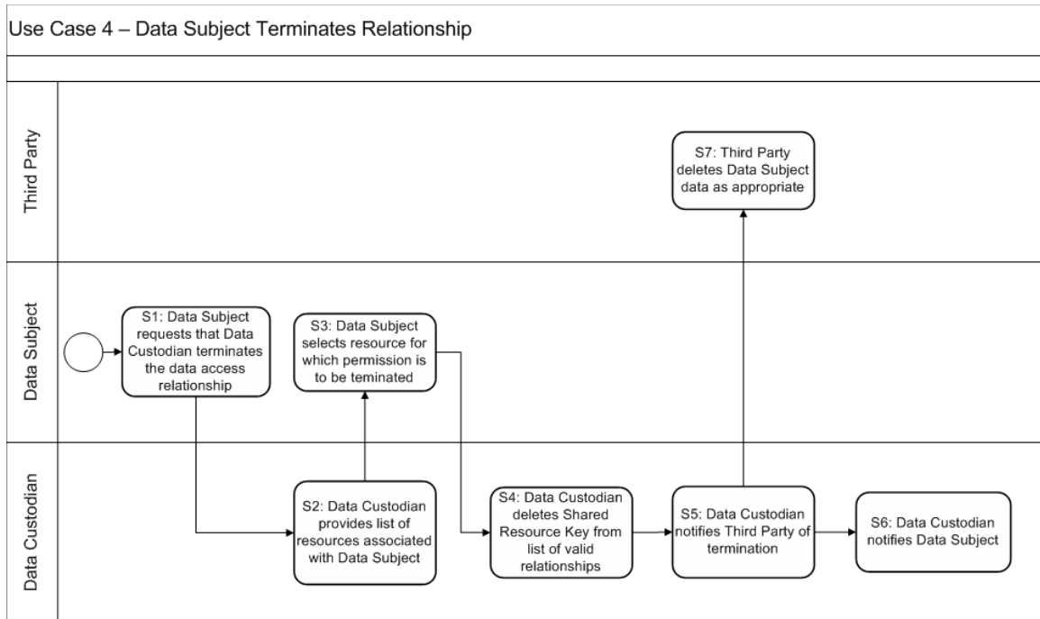
Diagram: Use Case 4 – Data Subject Terminates Relationship
