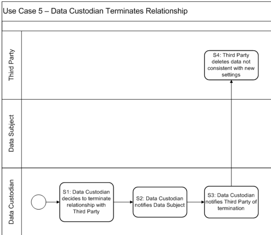
Diagram: Use Case 5 – Data Custodian Terminates Relationship
