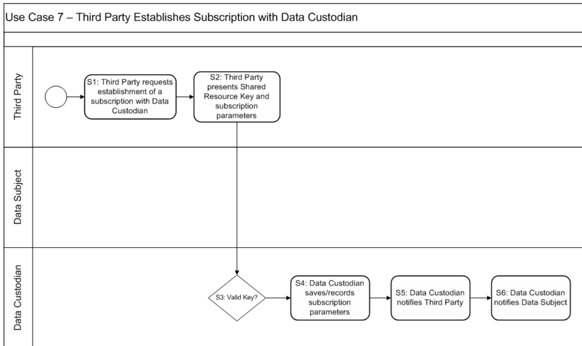
Diagram: Use Case 7 – Third Party Establishes Subscription with Data Custodian
