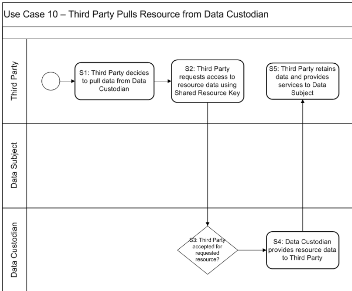
Diagram: Use Case 10 – Third Party Pulls Resource from Data Custodian
