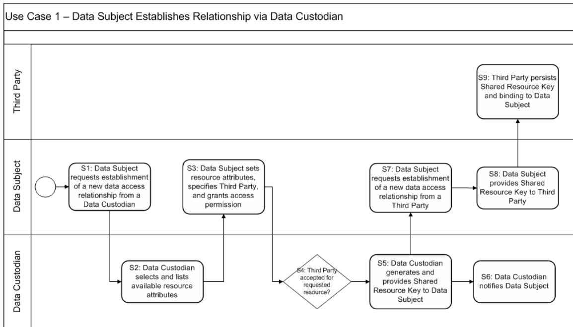
Diagram: Use Case 1 – Data Subject Established Relationship via Data Custodian
