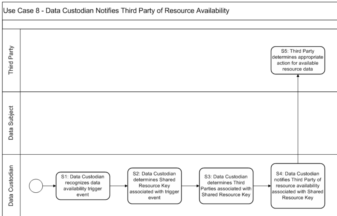
Diagram: Use Case 8 – Data Custodian Notifies Third Party of Resource Availability
